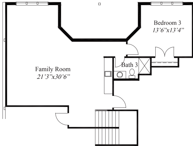
LOWER LEVEL 858 SQ.FT.
