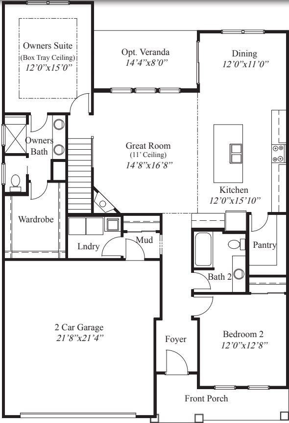
FIRST FLOOR 1,503 SQ.FT.
