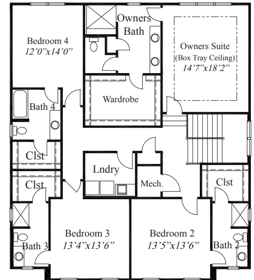
SECOND FLOOR 1,888 SQ.FT.
