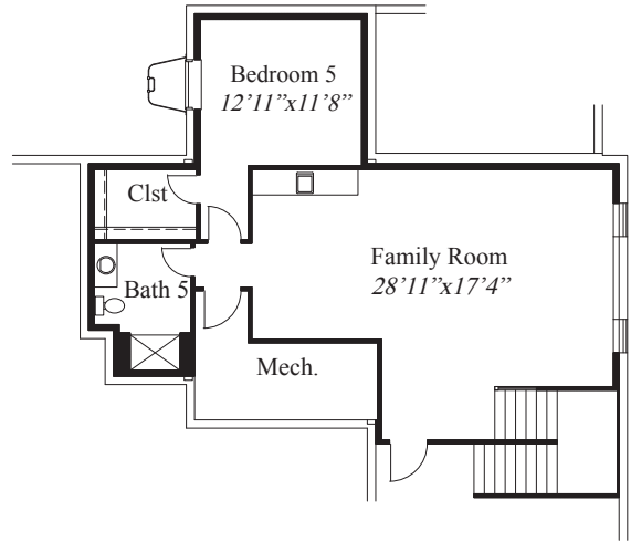
LOWER LEVEL 886 SQ.FT.
