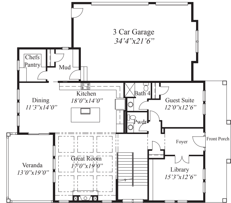
FIRST FLOOR 1,759 SQ.FT.
