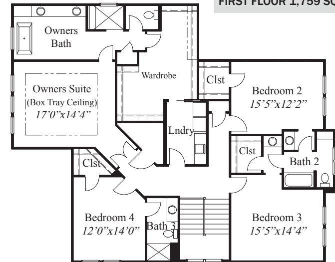
SECOND FLOOR 1,905 SQ.FT.
