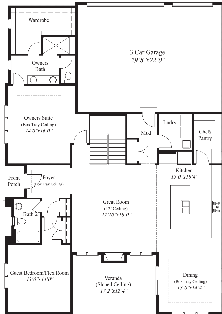
FIRST FLOOR 1,970 SQ.FT.
