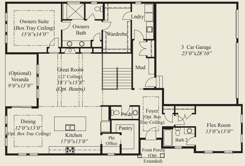
FIRST FLOOR 2,083 SQ.FT.
