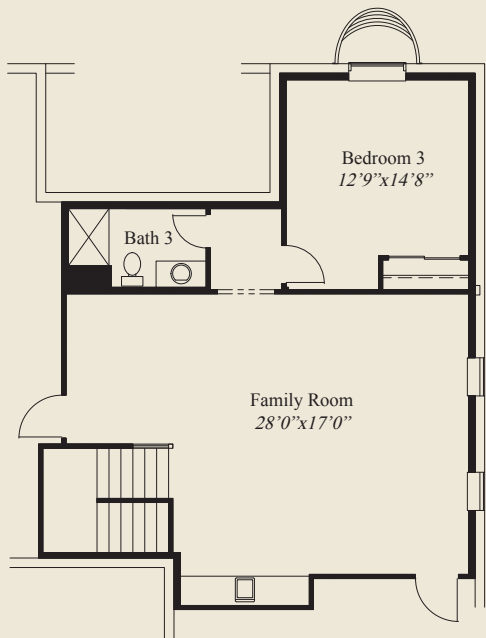
OPTIONAL FINISHED LOWER LEVEL 835 SQ.FT.
