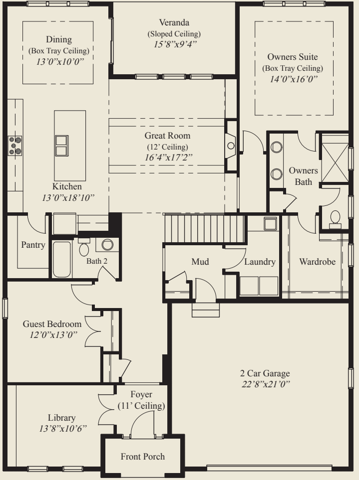
FIRST FLOOR 2,000 SQ.FT.
