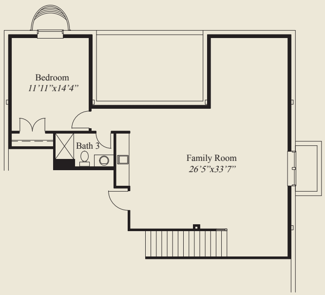
LOWER LEVEL 972 SQ.FT.
