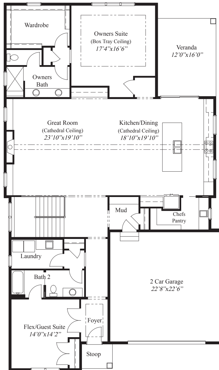
FIRST FLOOR 2,370 SQ.FT.
