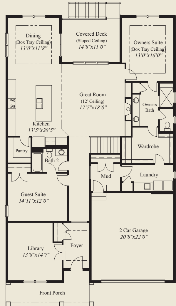
FIRST FLOOR 2,193 SQ.FT.
