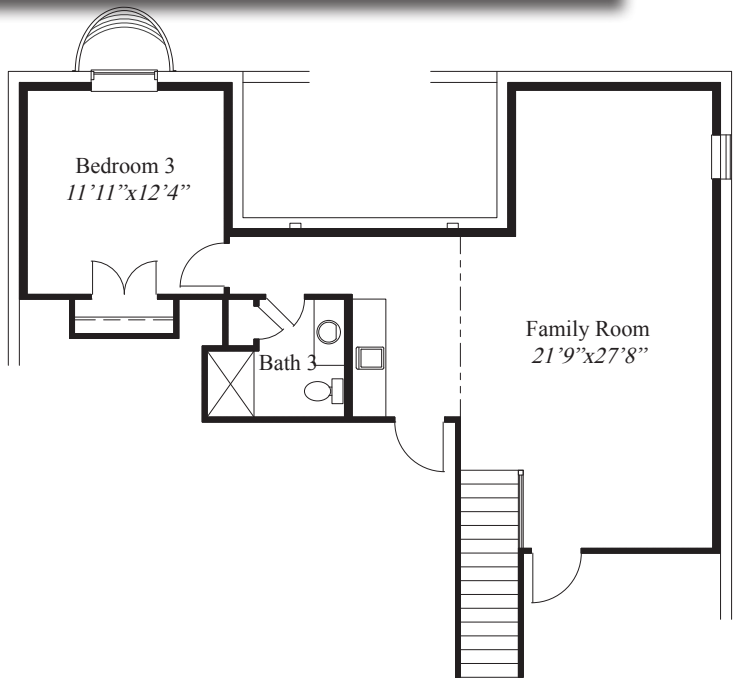
LOWER LEVEL 768 SQ.FT.
