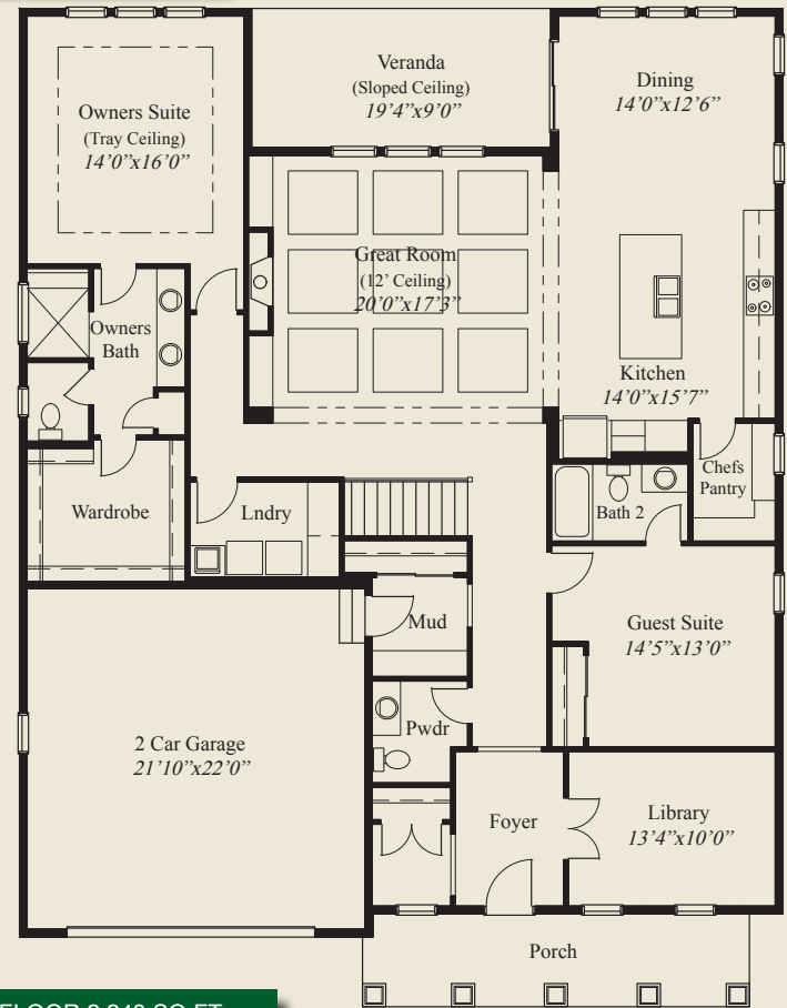
FIRST FLOOR 2,243 SQ.FT.
