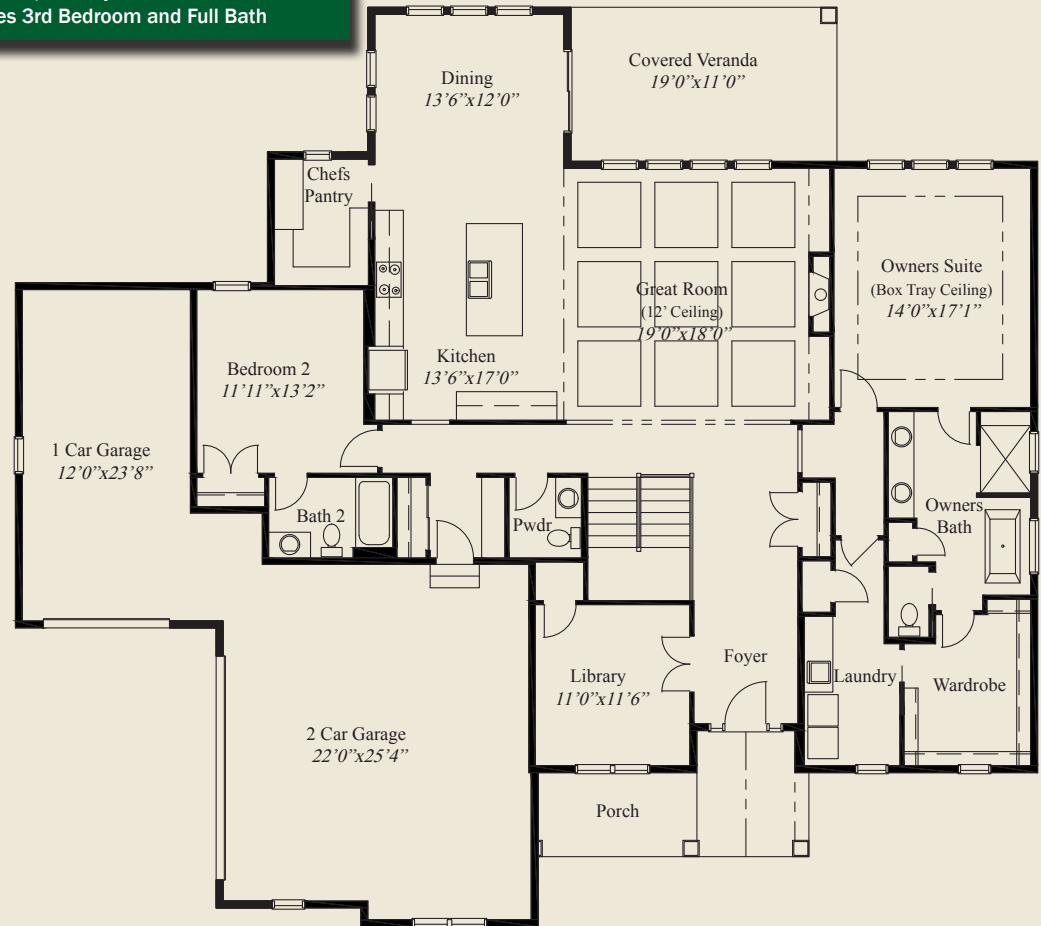
FIRST FLOOR 2,359 SQ.FT.
