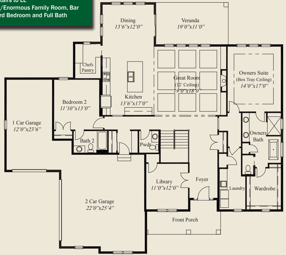
FIRST FLOOR 2,359 SQ.FT.
