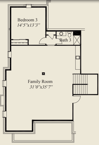
FINISHED LOWER LEVEL 1,316 SQ.FT.
