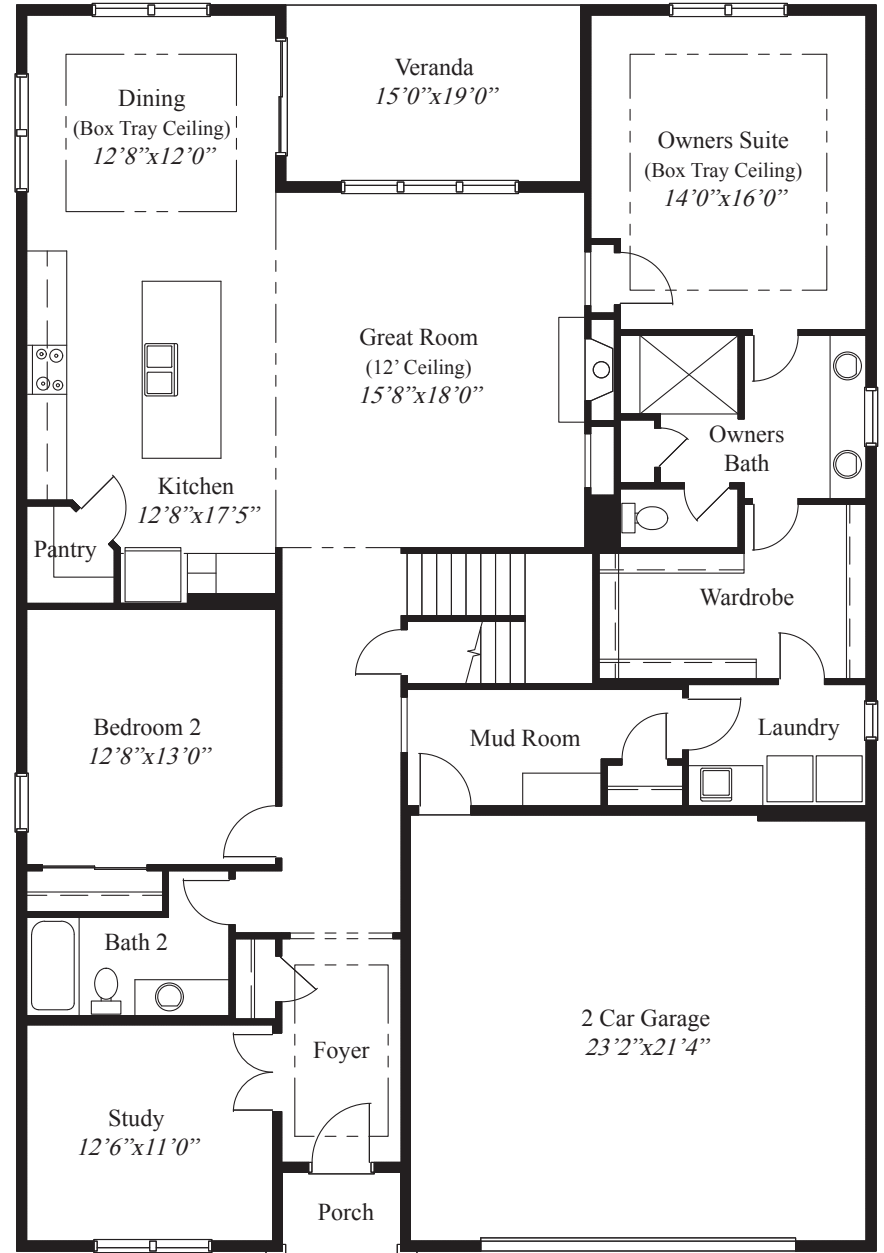
FIRST FLOOR 2,082 SQ.FT.
