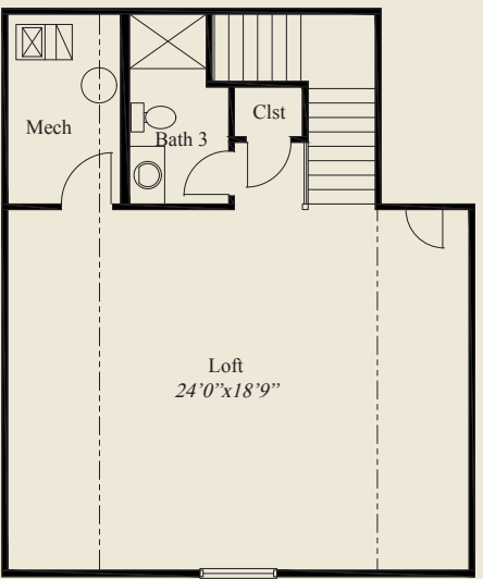
SECOND FLOOR 677 SQ.FT.
