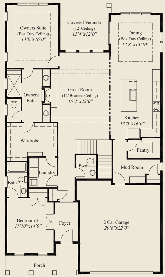
FIRST FLOOR 1,971 SQ.FT.
