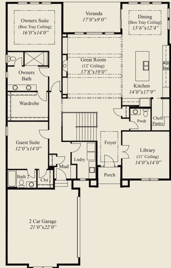
FIRST FLOOR 2,441 SQ.FT.
