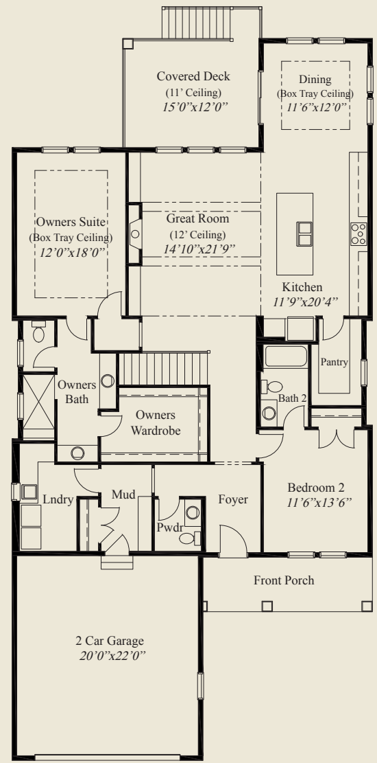
FIRST FLOOR 1,915 SQ.FT.
