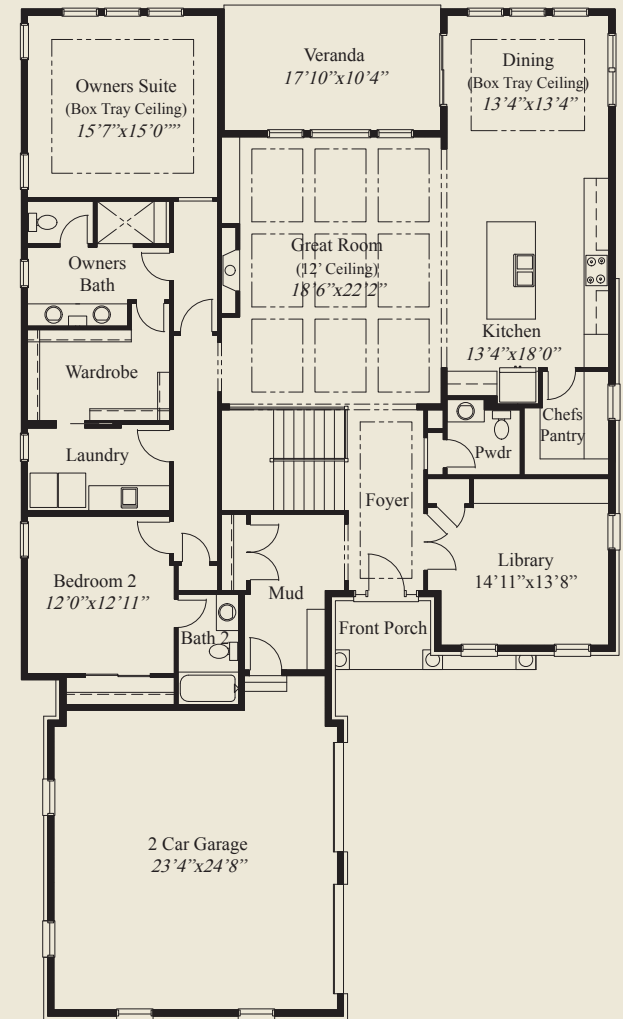
FIRST FLOOR 2,459 SQ.FT.
