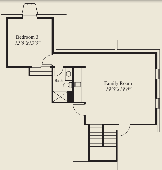
OPTIONAL FINISHED LOWER LEVEL 704 SQ.FT.
