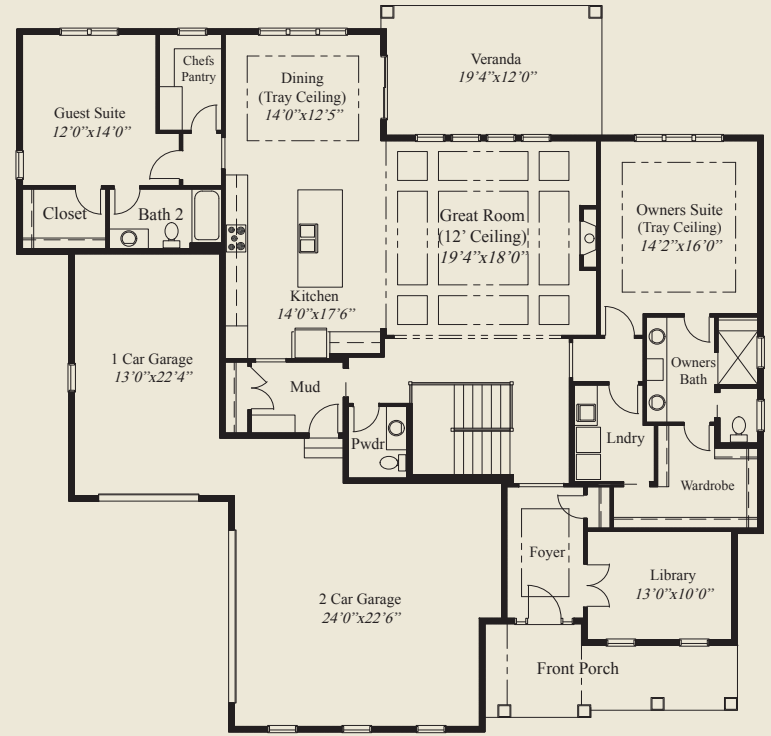
FIRST FLOOR 2,363 SQ.FT.
