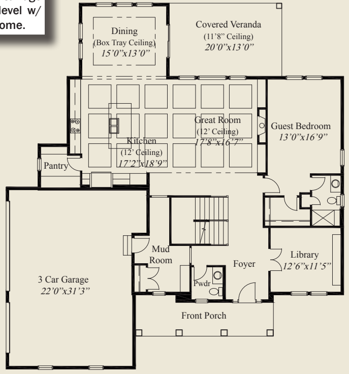
FIRST FLOOR 1,949 SQ.FT.
