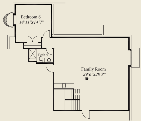
LOWER LEVEL 1,127 SQ.FT.
