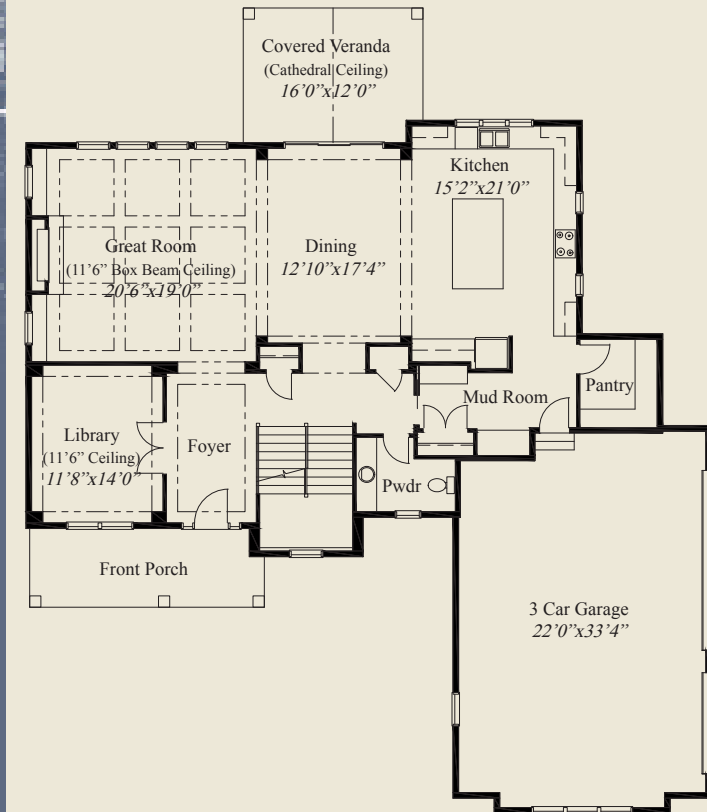
FIRST FLOOR 1,735 SQ.FT.
