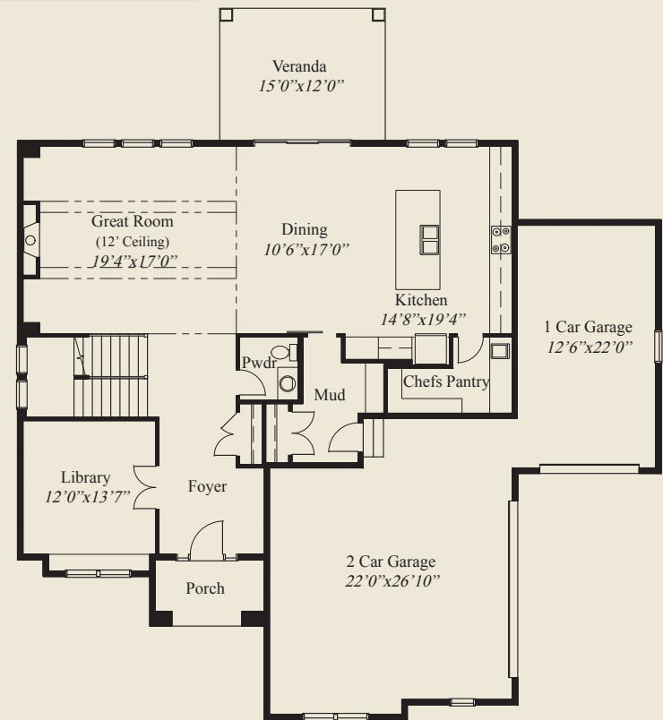
FIRST FLOOR 1,682 SQ.FT.
