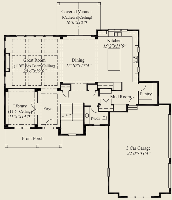
FIRST FLOOR 1,735 SQ.FT.
