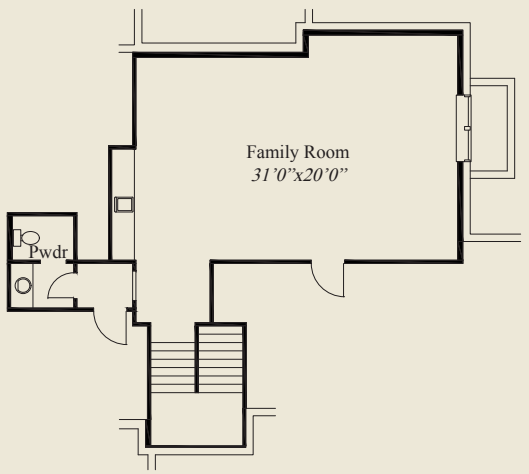
LOWER LEVEL 740 SQ.FT.
