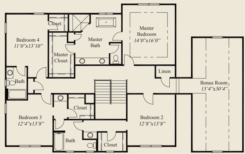
SECOND FLOOR 2,155 SQ.FT.
